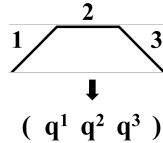
Figure 1. Rough correspondence between the articulatory phases of Articulatory Phonology and the quantized subsegments of Q Theory
