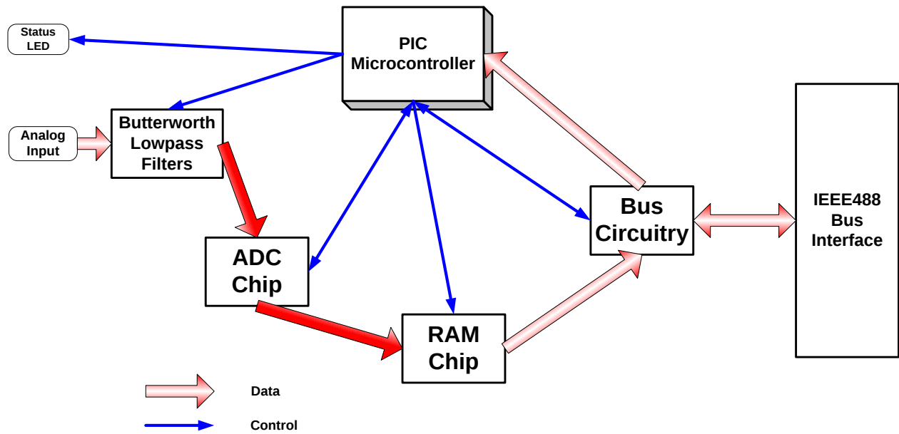
Block Diagram
