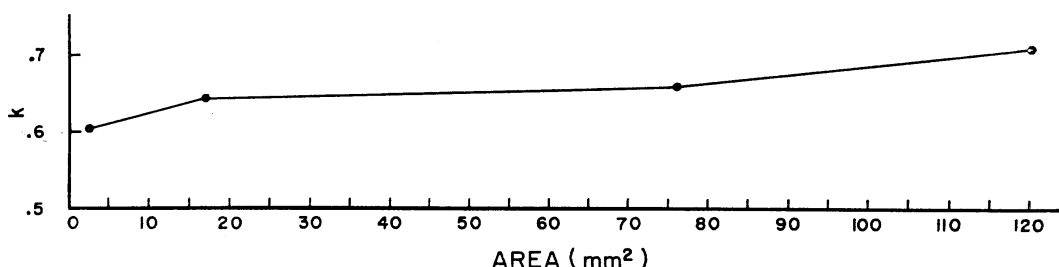
FIGURE 2. Relationship between orifice size and coefficient k . Since k varies so slightly with orifice size its average value (.65) is used as a constant for the orifice equation.
